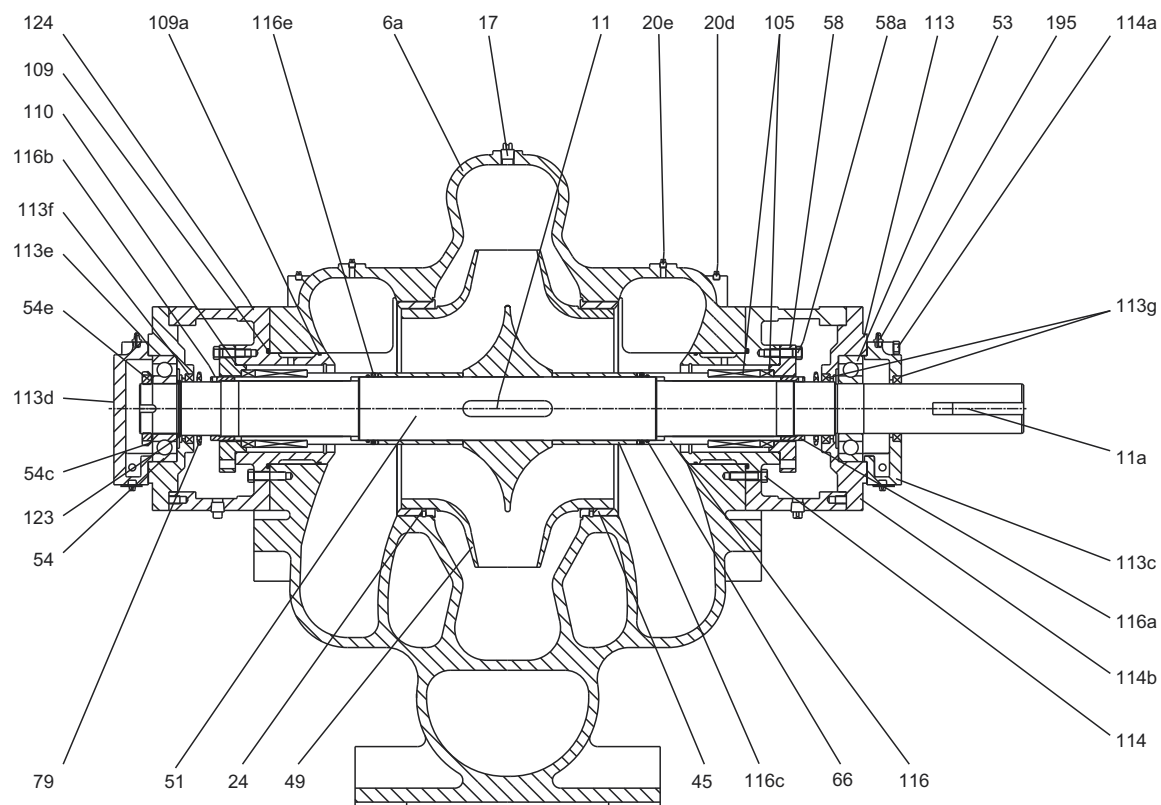
Fig. 13 Sectional drawing, optional construction type 2
