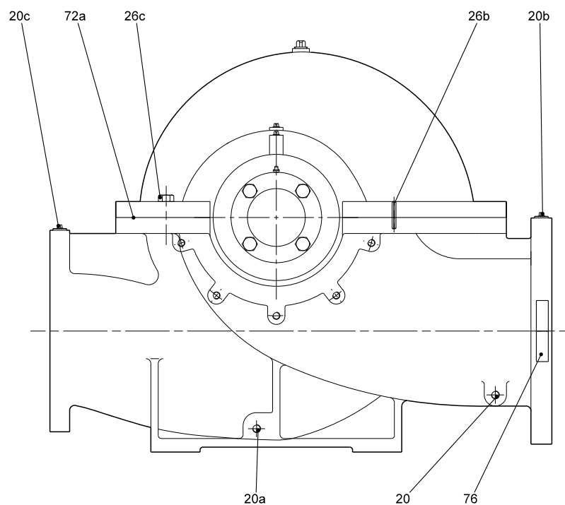
Fig. 14 Typical end view (non-drive end)
