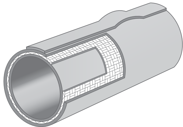
Figure 69 Cross-section of wellmaster hose
