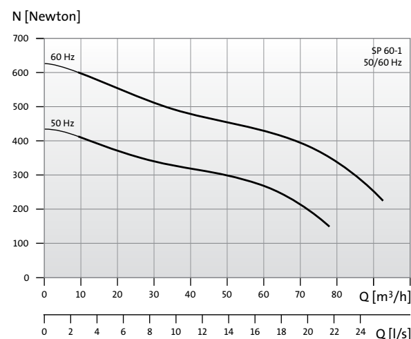
Figure 25 Single-stage axial-load curve, SP 60
