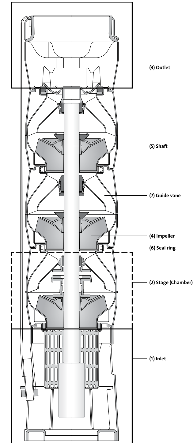
Figure 24 Submersible pump principle
