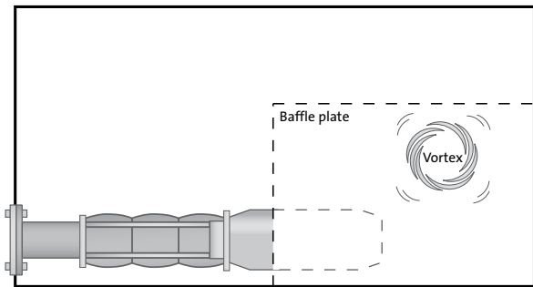
Figure 12 Vortex baffle plate on horizontally-installed pump (seen from above)
