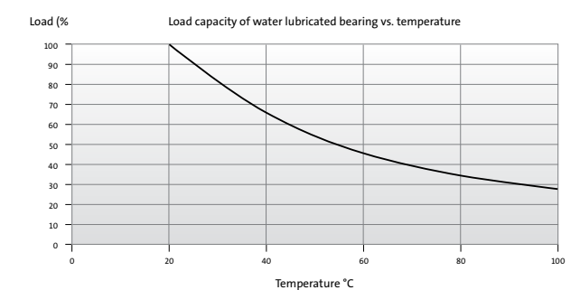
Figure 45 Diagram: Journal bearings load capacity as function of motor liquid temperature.
