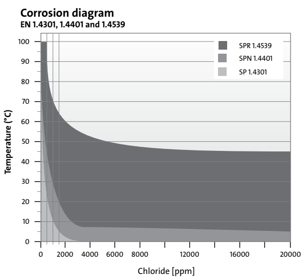
Figure 22 Corrosion diagram
