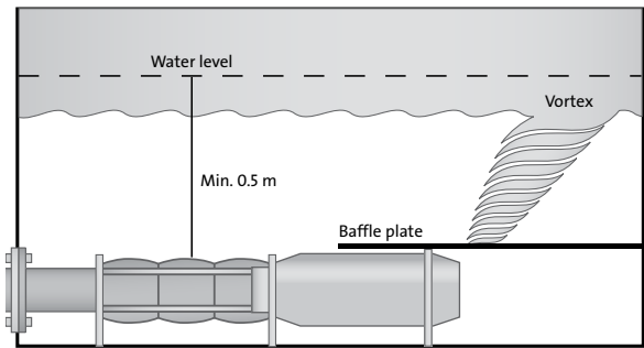
Figure 13 Vortex baffle plate on horizontally installed pump (cross-section)
