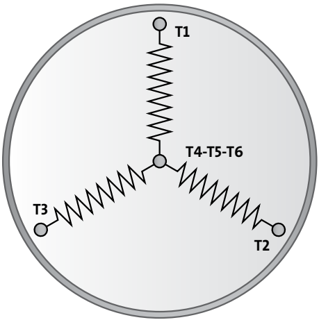
Figure 32. Wye configuration at start-up
