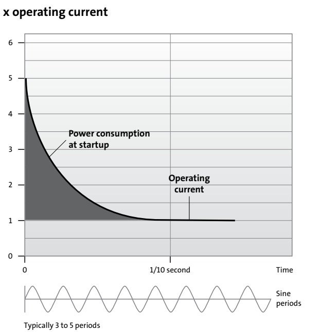
Figure 30 Current flow by DOL starting
