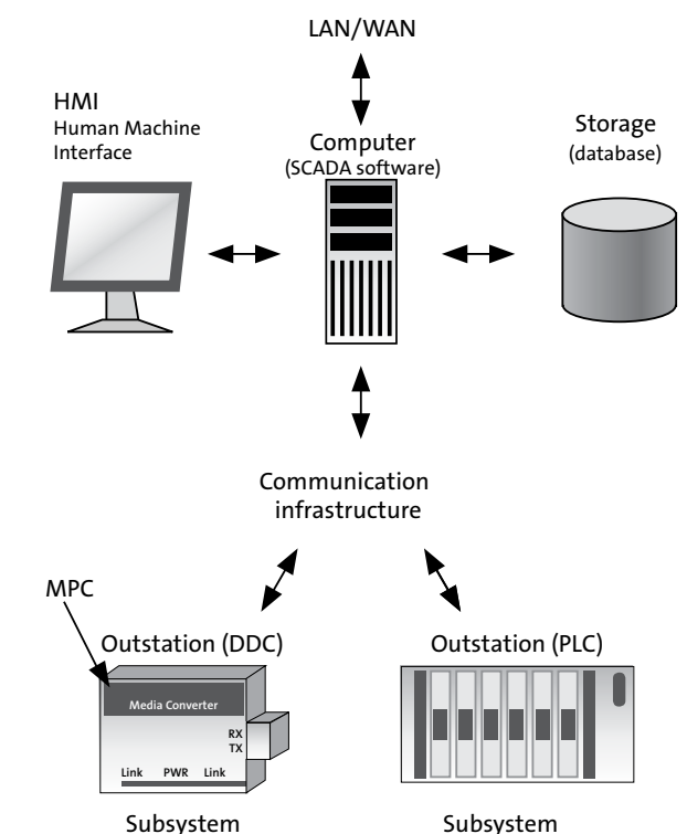
Figure 61 Illustration of the main parts of a SCADA system
