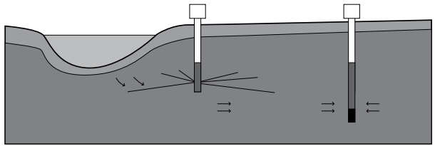
Figure 2 Riverside well installations
