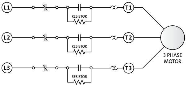
Figure 36. Typical electrical diagram for a primary resistor reduced voltage starter
