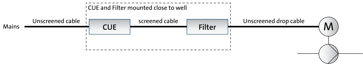
Figure 42 Submersible pump without connection box
