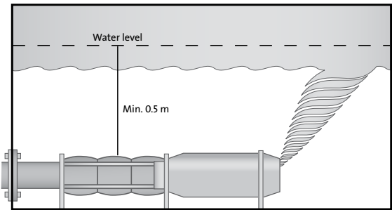
Figure 11 Flow sleeve on horizontally installed pump
