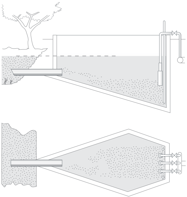
Figure 8 Settling tank principle
