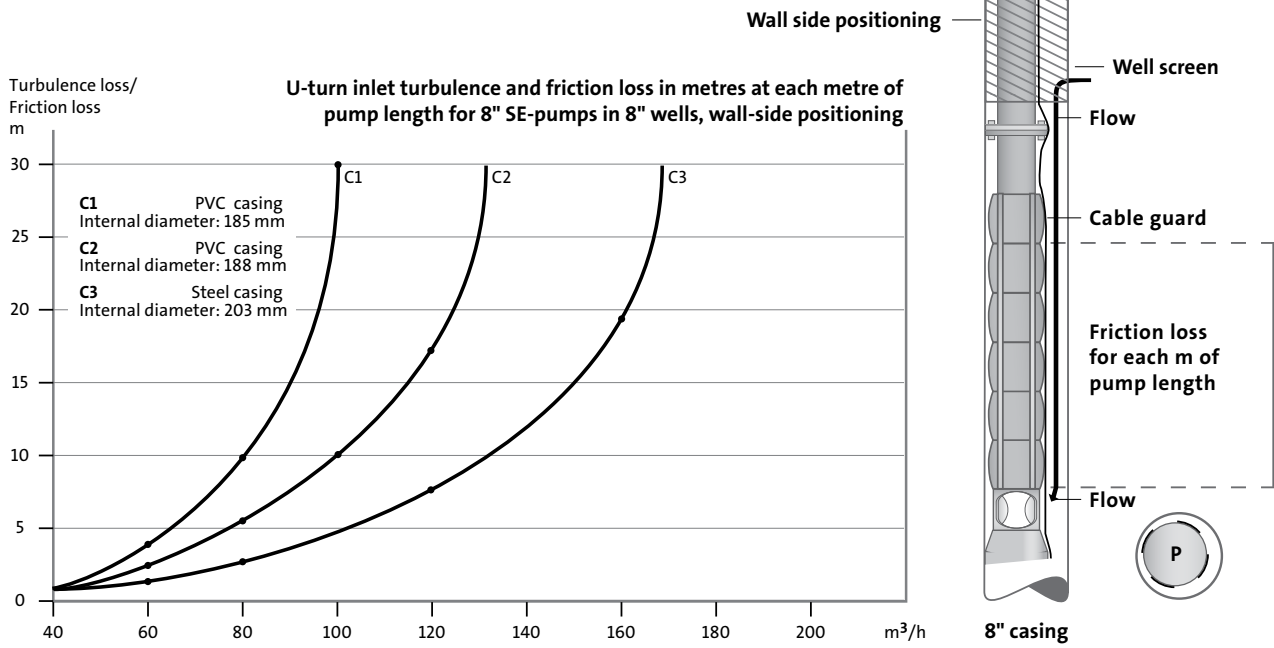
Figure 55 U-turn, 8"
