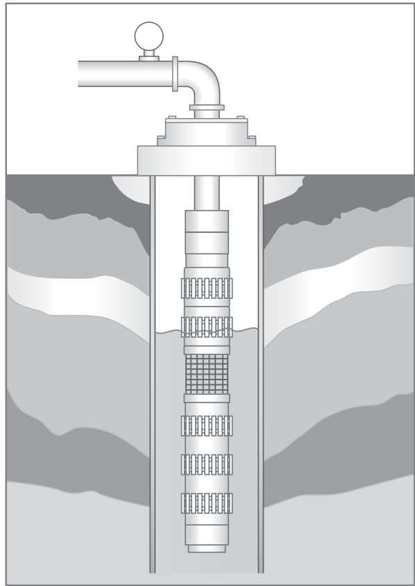
Figure 67 Submersible pump set with sacrificial zinc anodes.
