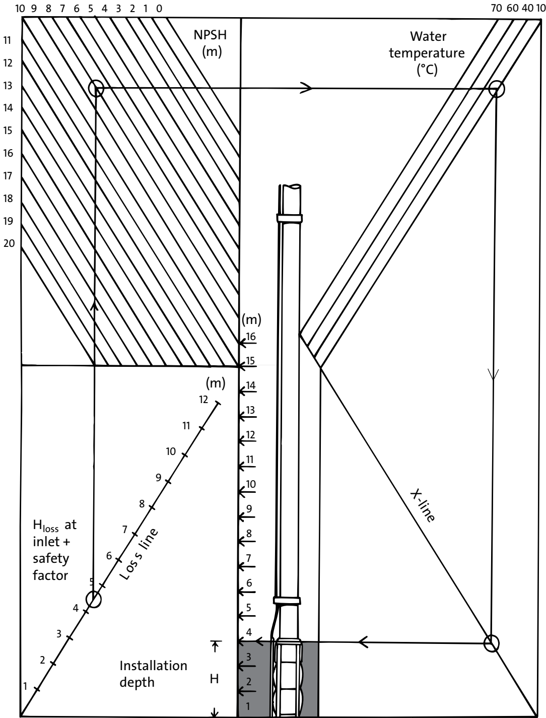
Figure 18 Diagram for quick calculation of minimum installation depth
