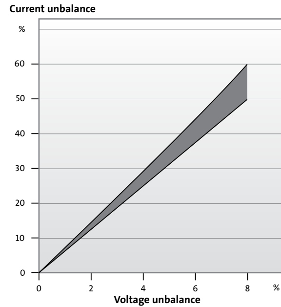
Figure 48 Relationship between voltage and current unbalance
