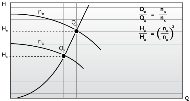
Figure 39 Pump performance with different frequencies
