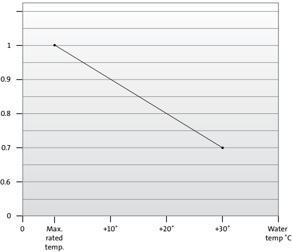
Figure 57 Derating of submersible motors
