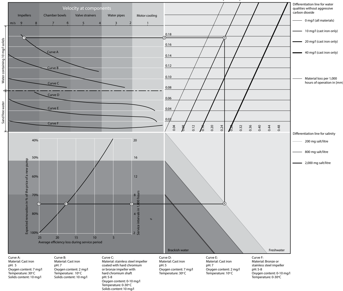
Figure 9 Recommended service intervals for submersible pumps
