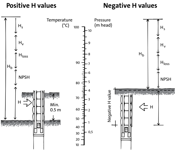
Figure 16 Installation depth
