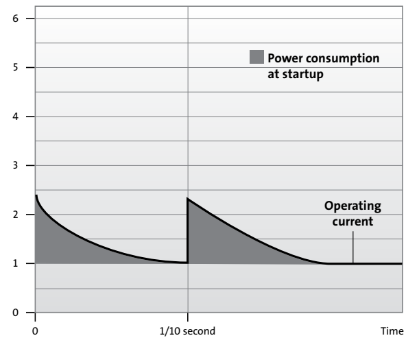
Figure 34 Current flow by autotransformer starting
