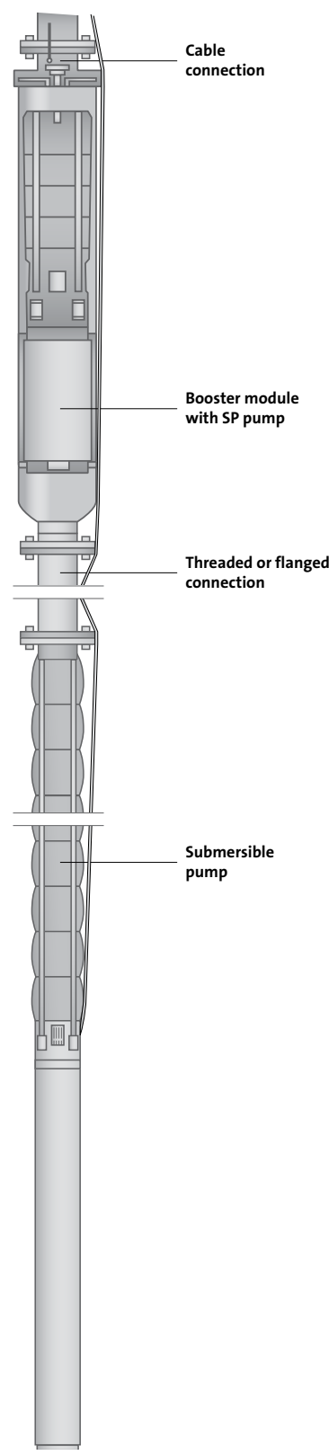
Figure 60 Series coupled submersible pump
