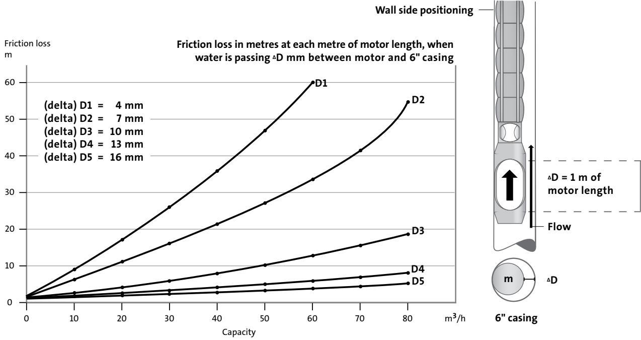
Figure 52 Friction loss, 6"
