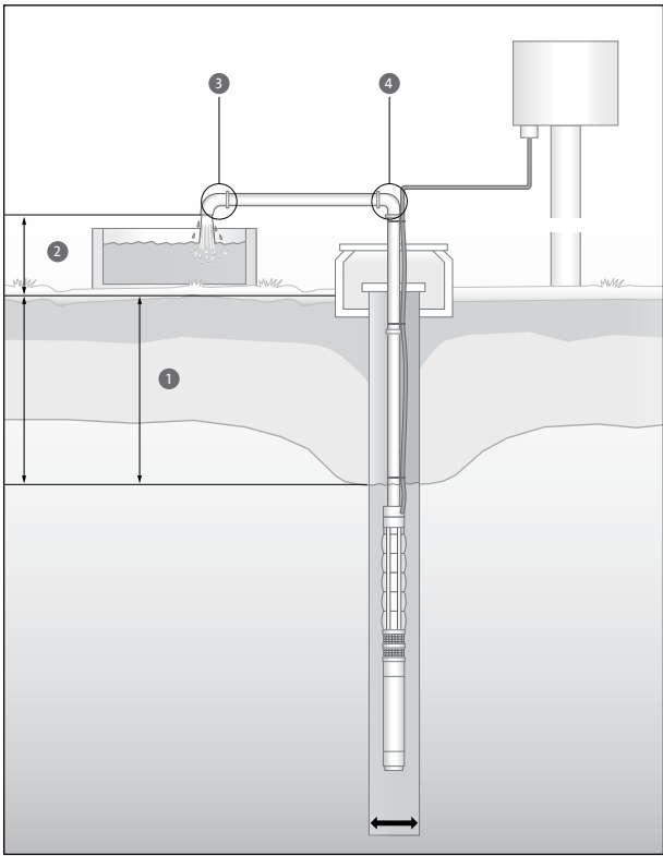
Figure 25 Total head calculation
