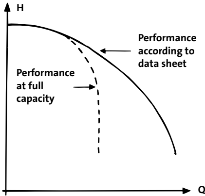
Figure 17 Performance reduction at cavitation
