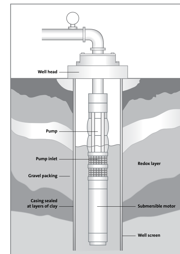
Figure 1 Groundwater well with submersible pump
