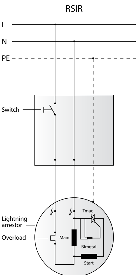
Figure 29 RSIR motor
