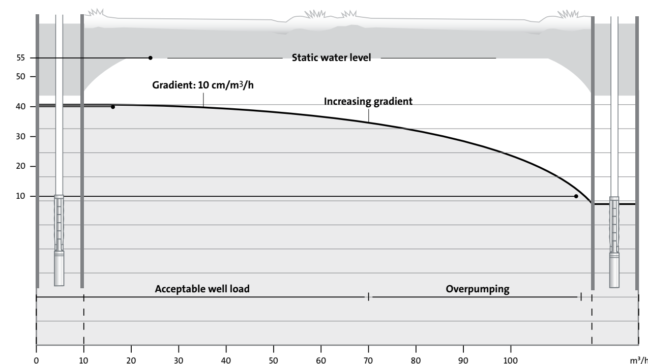
Figure 7 Dynamic water-level variations by test pumping
