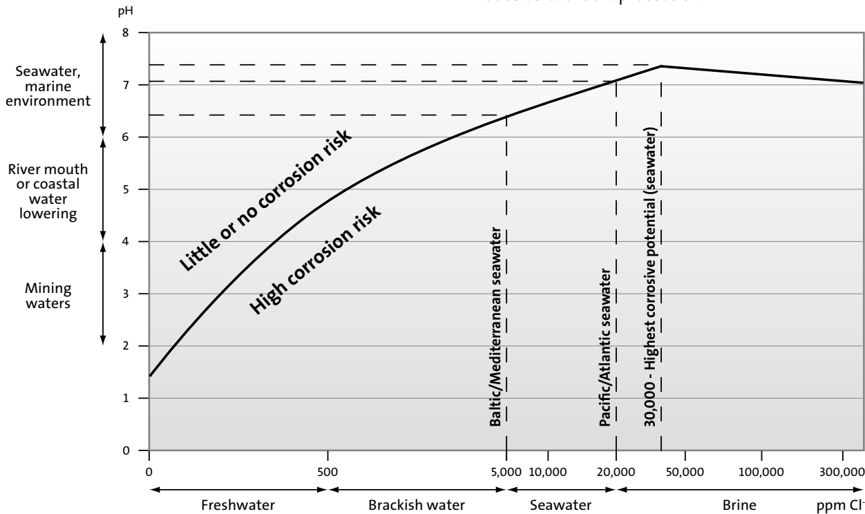
Figure 10 Corrosion due to chlorides
