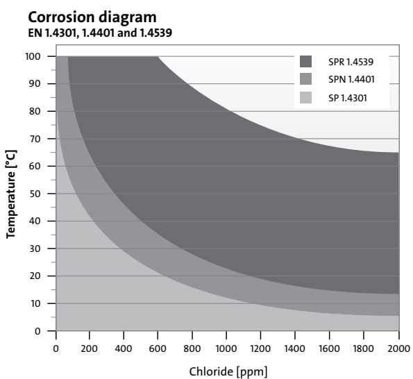
Figure 21 Corrosion diagram
