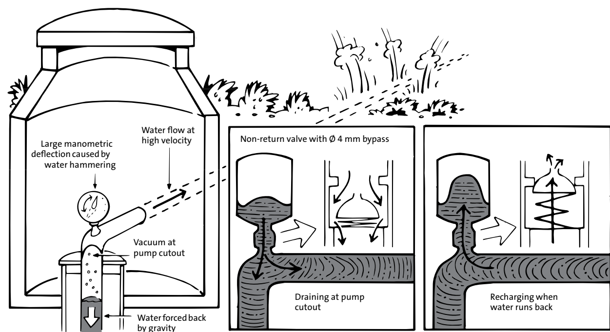
Figure 19 Elimination of water hammer
