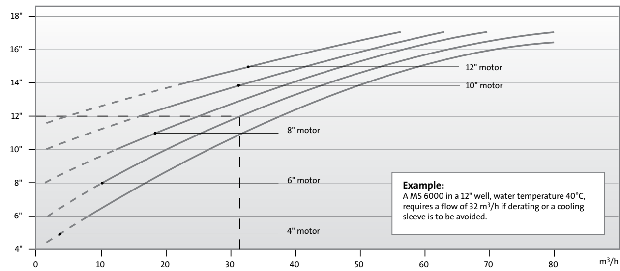
Figure 56 Maximum full-load cooling water temperature
