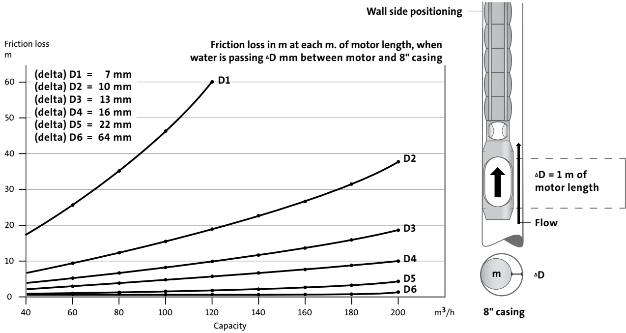
Figure 53 Friction loss, 8"
