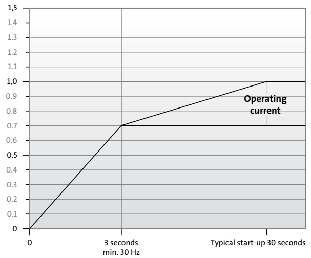
Figure 40 Current flow by frequency converter starting
