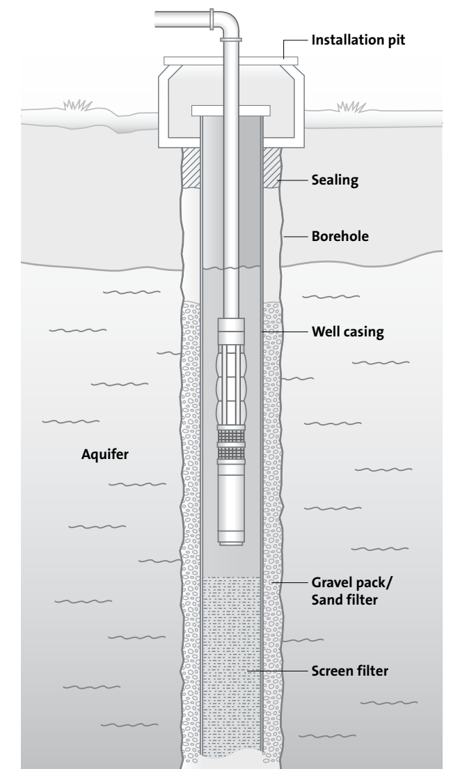
Figure 50 Typical groundwater well components
