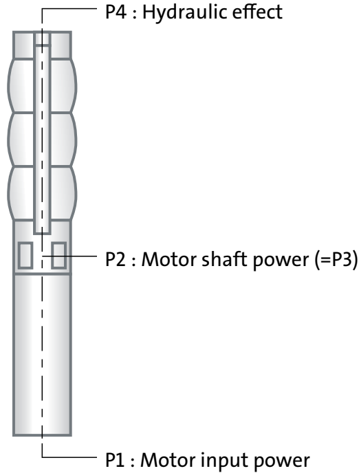
Figure 26 Power definitions
