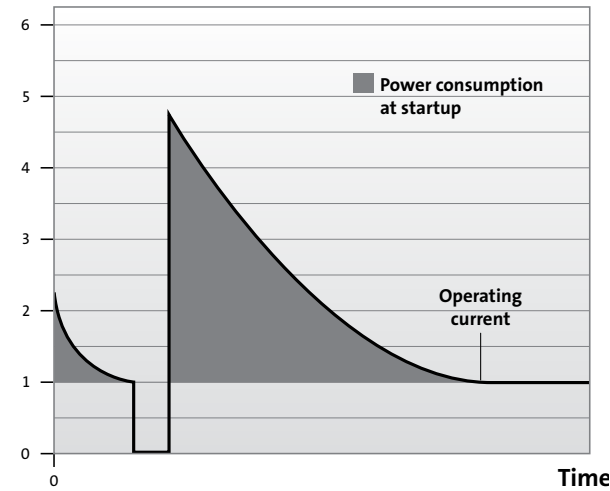
Figure 31 Current flow by SD starting
