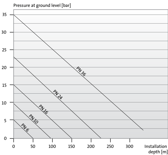
Figure 59 Required pipe pressure class at different installation depths and actual pressure at ground level
