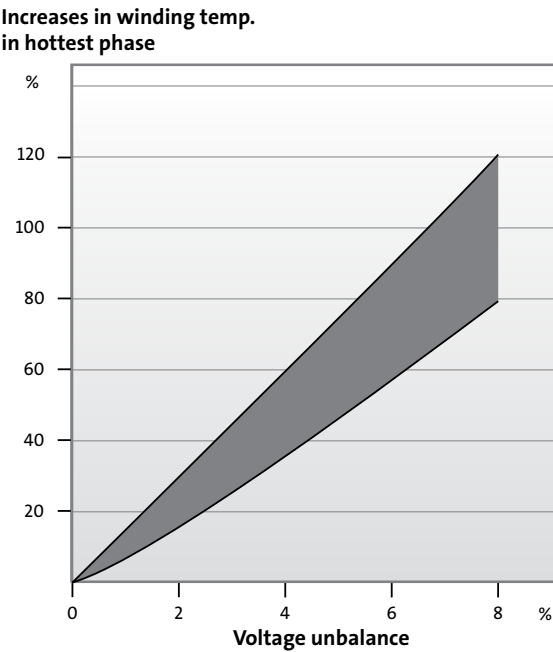
Figure 49 Relationship between voltage unbalance and temperature
