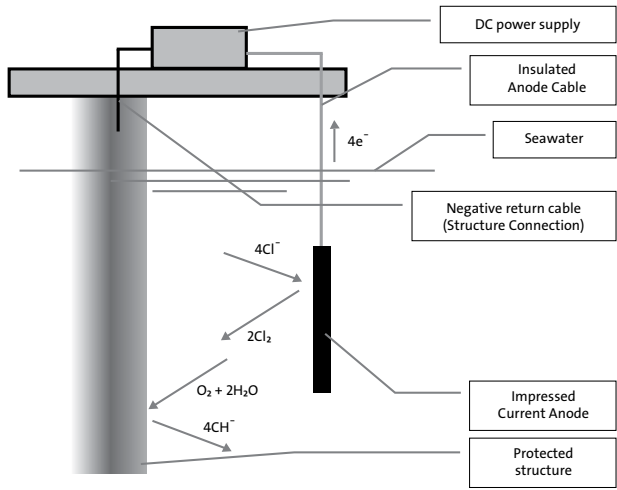
Figure 68 Principle of impressed current cathodic system
