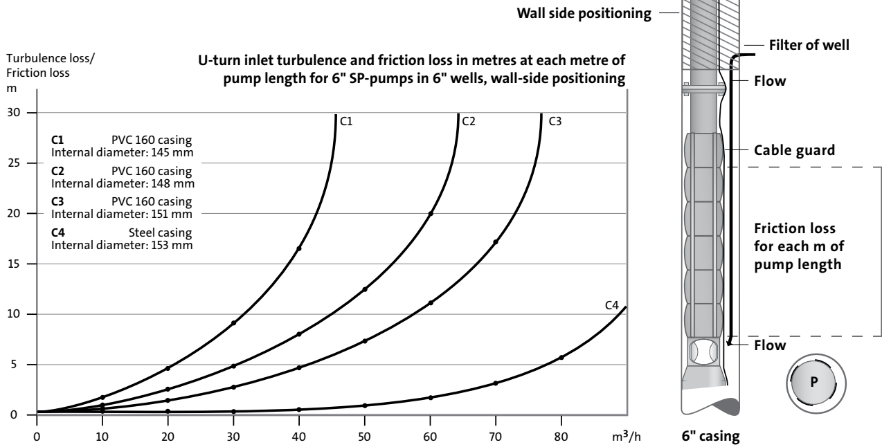
Figure 54 U-turn, 6"
