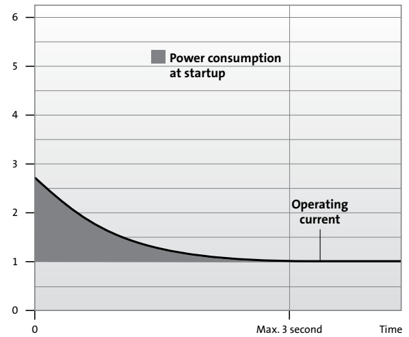
Figure 38 Current flow by soft starting
