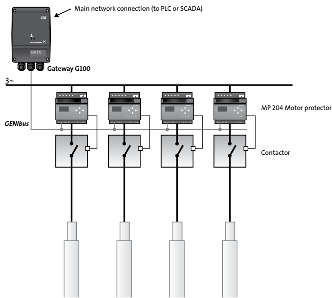
Figure 66 Illustration of the remote monitoring and control of SP pump installations
