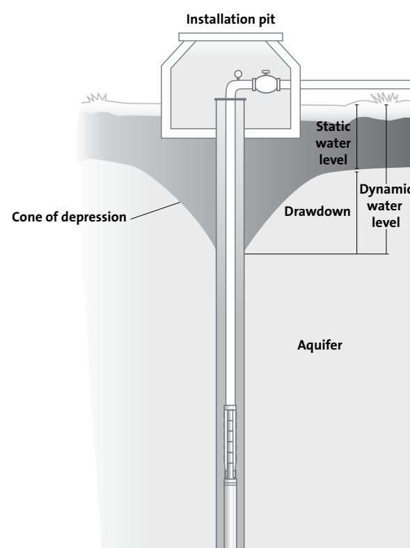
Figure 51 Static and dynamic water level
