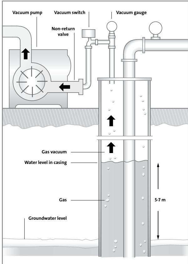
Figure 15 Vacuum wells
