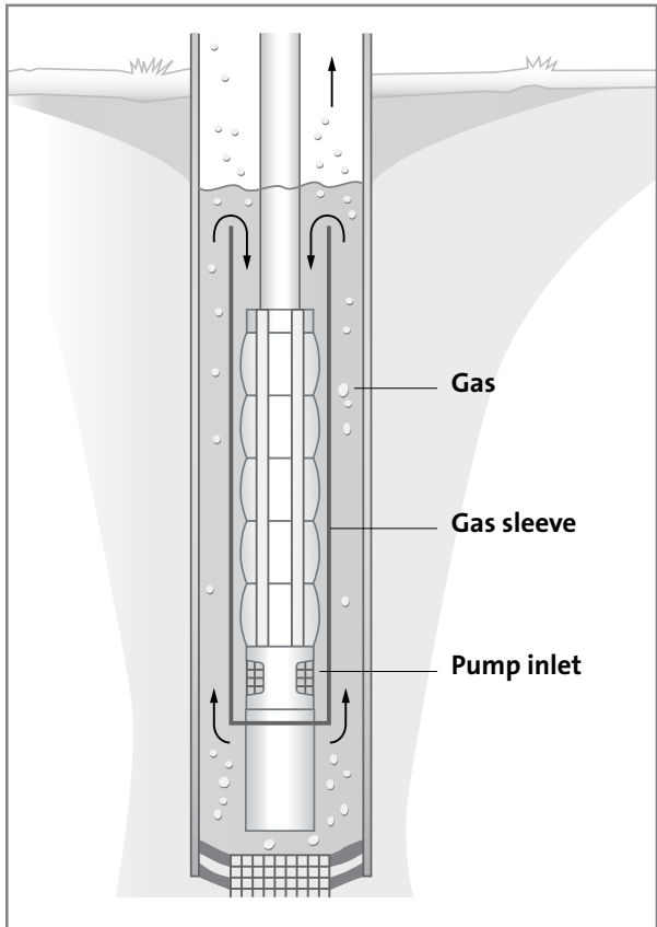
Figure 14 Gas evacuation
