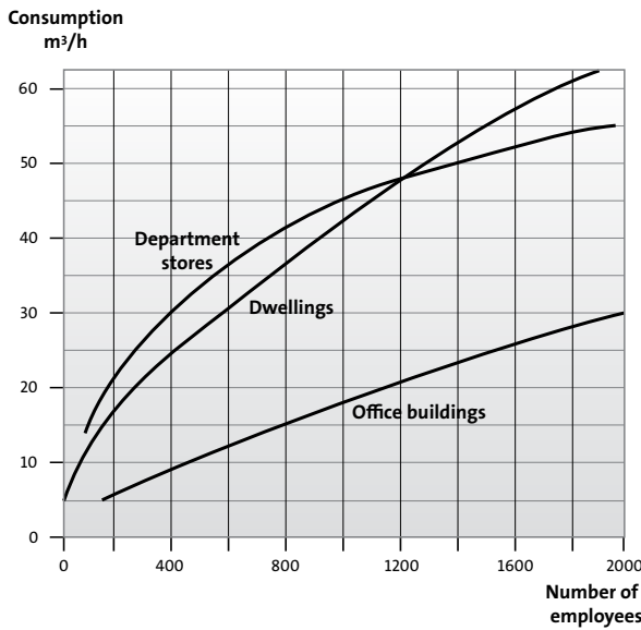
Figure 5 Peak water consumption
