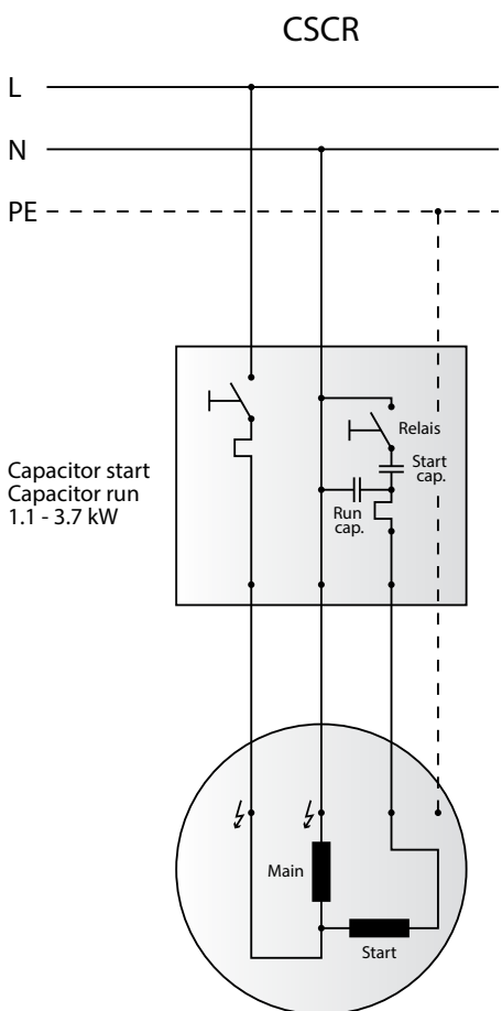
Figure 28 Schematic diagram of a CSCR motor
