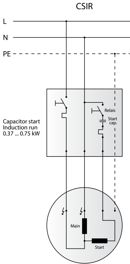
Figure 27 Schematic diagram of a CSIR motor
