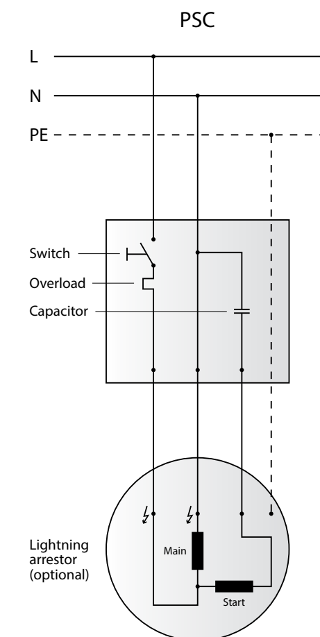
Figure 26 PSC
