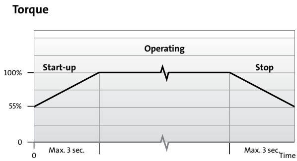
Figure 37 Recommended start-up and stop time, max. 3 sec.
