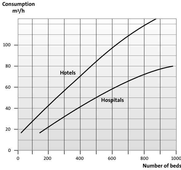
Figure 4 Peak water consumption
