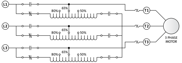
Figure 35 Typical electrical diagram for an autotransformer reduced voltage starter
