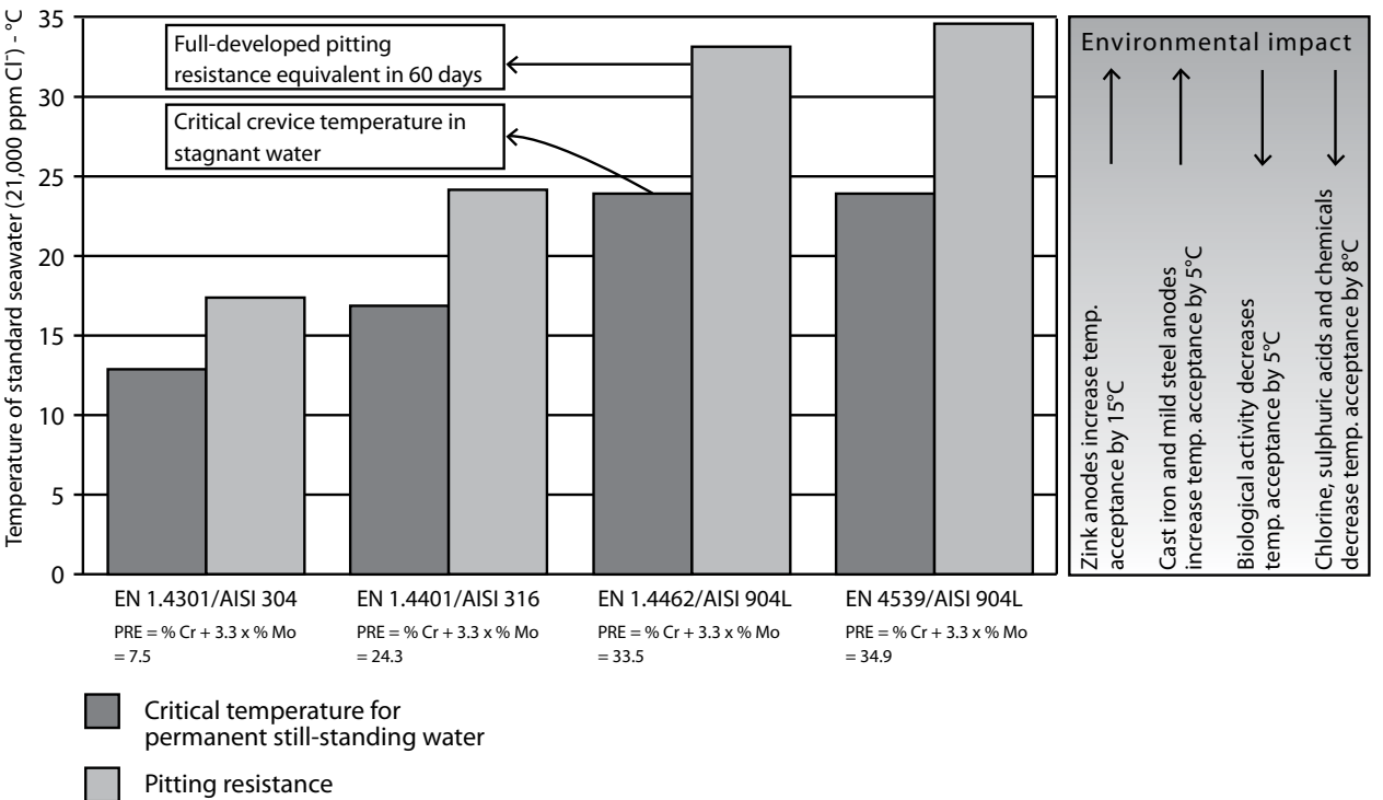
Figure 20 Corrosion resistance
