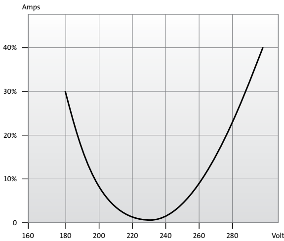
Figure 46 Current variation as a function of over- and undervoltage on a 230 V motor.
