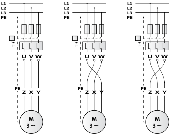
Figure 47 Optimal connection
